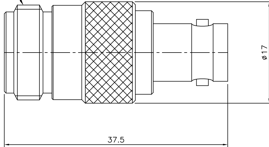
N JACK to BNC JACK-Adaptor (75 OHm)
