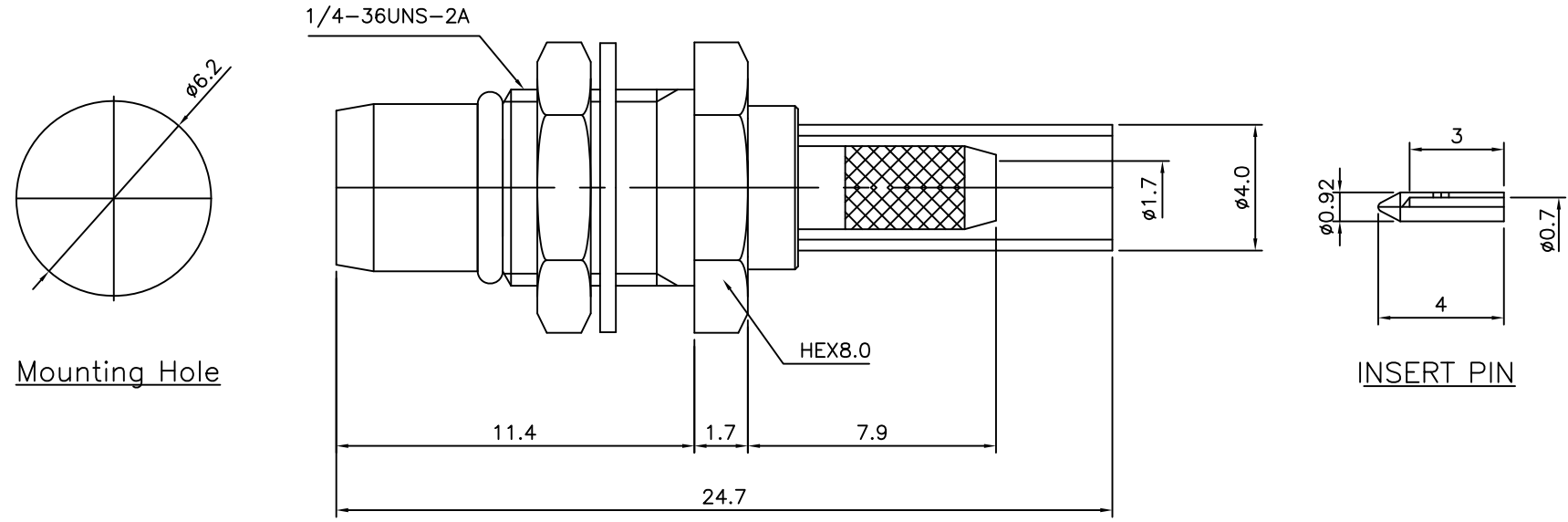
BMA-Straight Bulkhead PLUG for Cable-RG316
