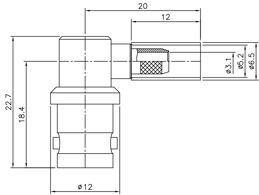
BNC Right Angle-JACK for Cable-RG58
