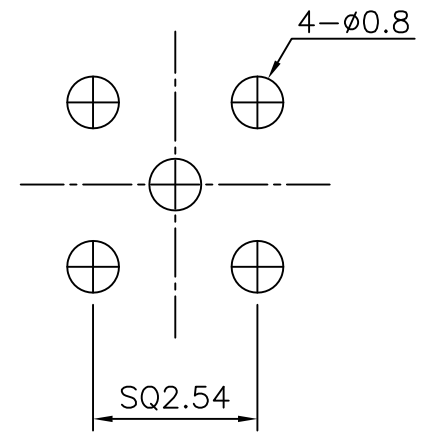
PCB MOUNT PLAN
