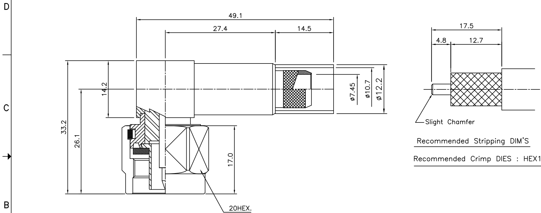
N-Right angle Plug for LMR400 Crimp Outer/Spring Finger Center
