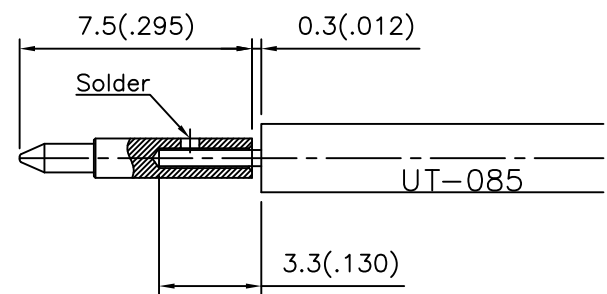
CENTER CONTACT
