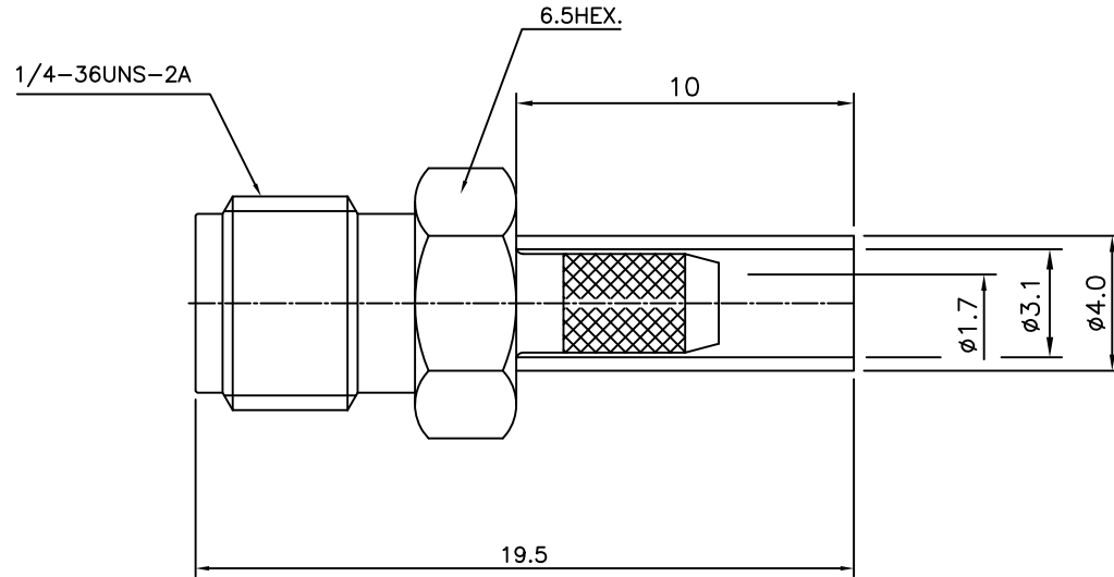
SMA-Straight-JACK for Cable:RG-316,174
