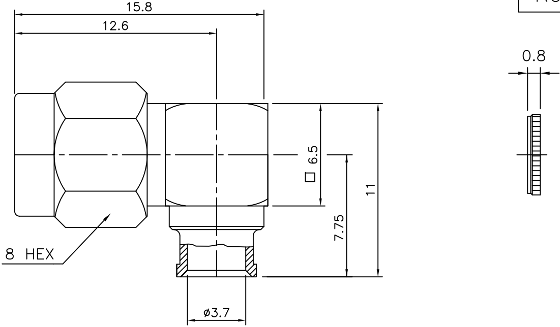
SMA-Right Angle-PLUG for Cable-UT141
