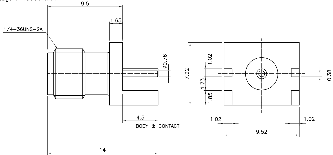
SMA PCB Edge Mount Jack Receptacle -Round Contact(1.60mm Board)
