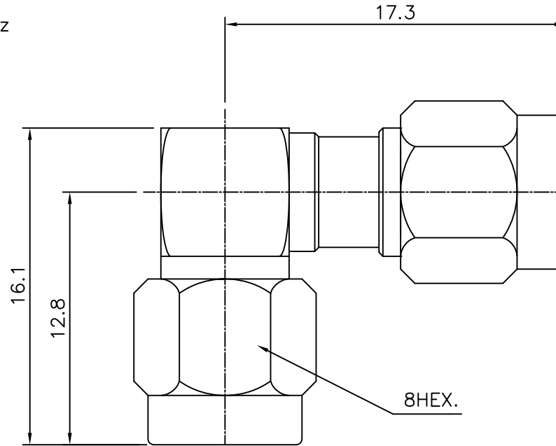
SMA Right Angle Plug to Plug Adaptor
