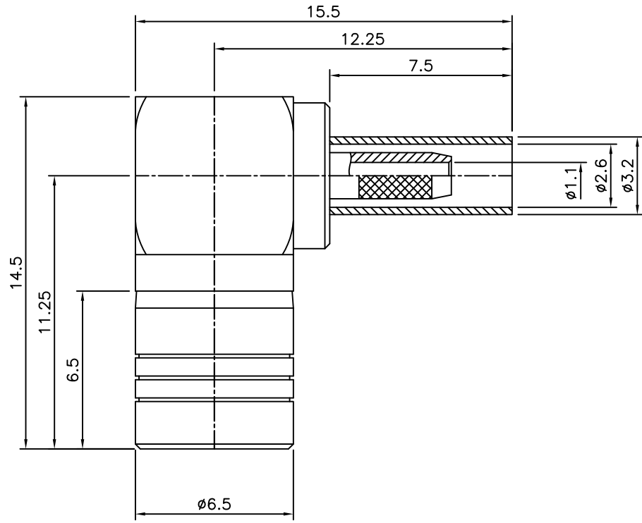
SMB-Right Angle-PLUG for Cable-RG178
