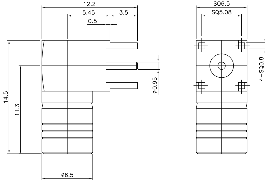
SMB-Right Angle PLUG PCB MOUNT
