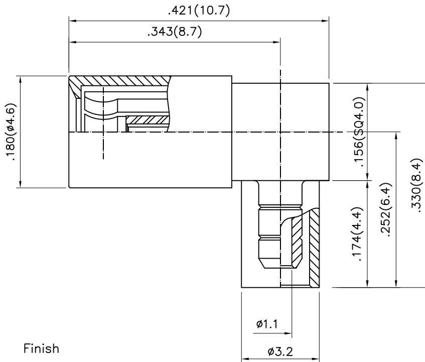
SSMB Right Angle Cable Plug for RG178
