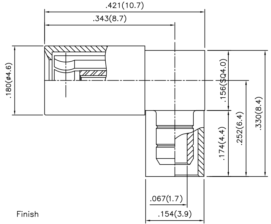
SSMB Right Angle Cable Plug for RG316,174
