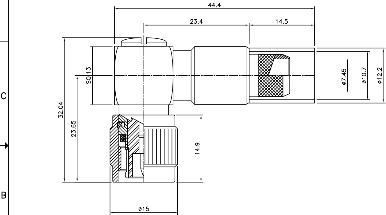
TNC Right anle Plug(No-solder) for LMR400/RG 8 Crimp Outer/Spring Finger Center
