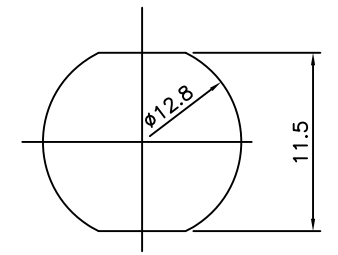
PANEL MOUNTING HOLES
