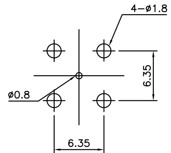
PCB MOUNTING HOLES
